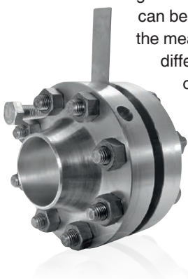
Orifice with flanged welding sockets
